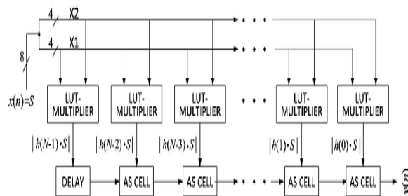
Figure 2 Conventional LUT-multiplier-based structure of an n-tap transposed form FIR
