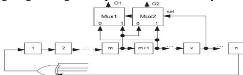
Fig. 1. Swapping arrangement for an LFSR.
