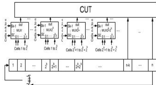
Figure 6: The Architecture of the RLFSR for test-per-clock BIST
