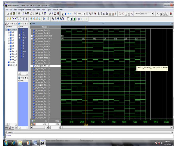
Fig.5. BS-LFSR Algorithm
