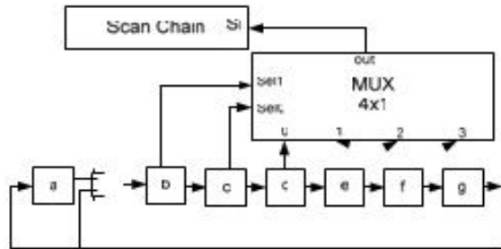
Figure 4: 7-bit internal LFSR with 4x1 multiplexer to get a smoothing degree k=2
