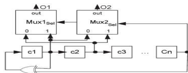
Fig. 2. External LFSR that implements the prime polynomial x^n + x + 1 and the proposed swapping arrangement.
