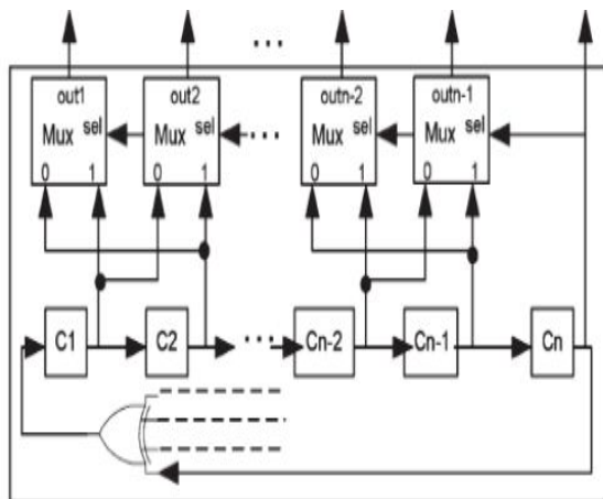
Fig. 3. BS-LFSR can be used to generate exhaustive patterns for test-per-clock BIST.
