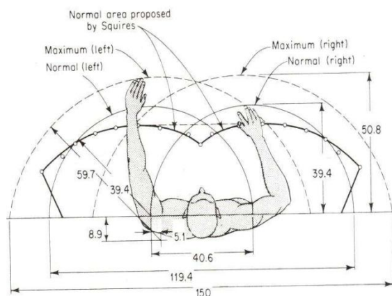
Fig. 1: Recommended working distance for the arms (Sanders and McCormick, 1993)
