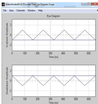
Figure 9: Rake receiver output with eye diagram after MLSE equalization.
