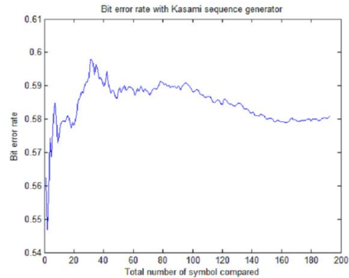
Figure 5: Rake output with Kasami sequence and random integer generator.
