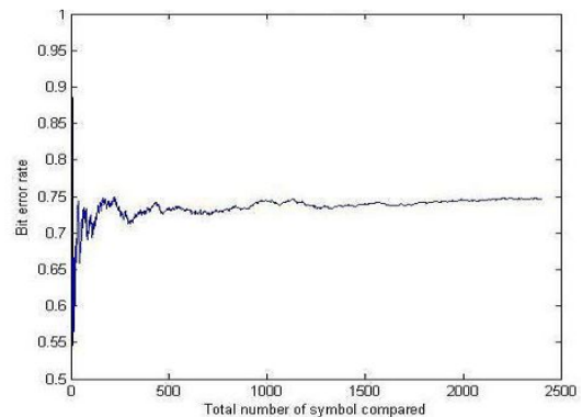
Figure 6: Rake output with Gold code sequence and random integer generator.
