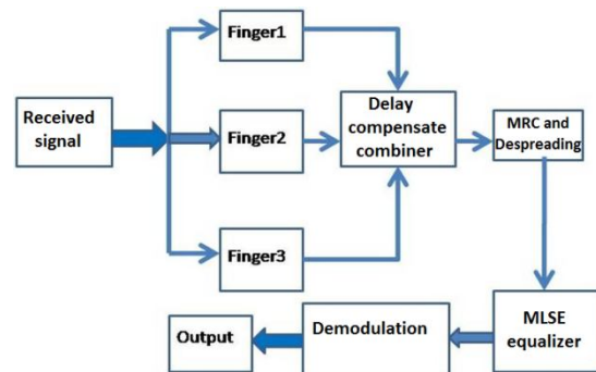
Figure 2: Proposed model of rake receiver.
