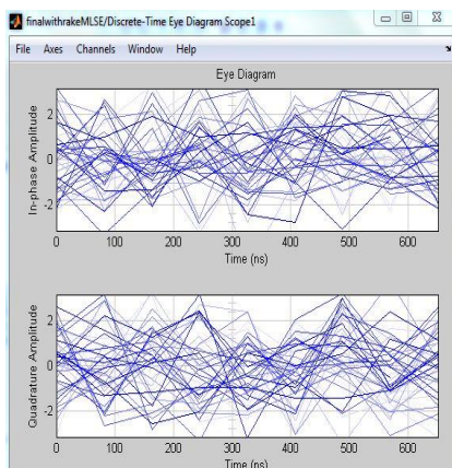
Figure 8: Rake receiver output with eye diagram before equalization.
