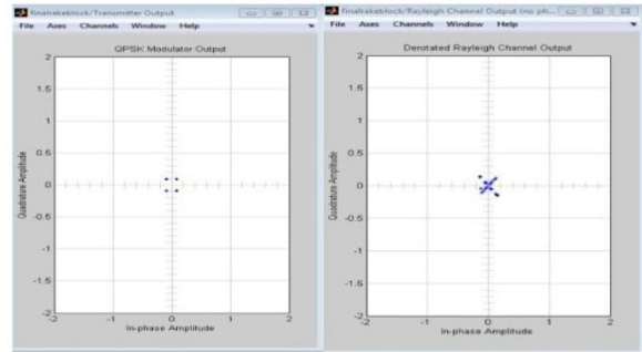
Figure 3: QPSK modulated & Rayleigh fading channel output
