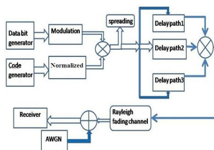
Figure 1: Block diagram of generic SSM transmitter.
