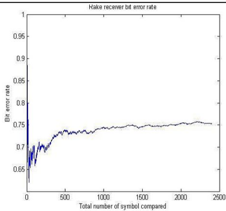
Figure 7: Rake output with PN- sequence and Random integer generator
