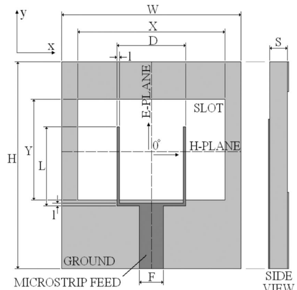
Fig.2 schematic view of wide slot
