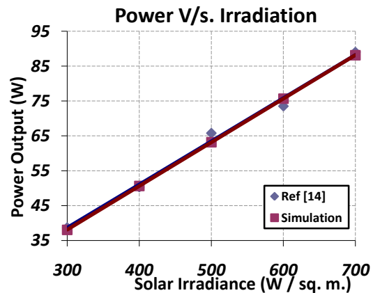
Figure 5. Relationship between the Electrical Power and Solar Irradiation at 25 o C.
