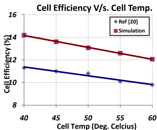
Figure 4. Relationship between the Electrical Efficiency and Cell Temperature at reference temperature of 25 o C
