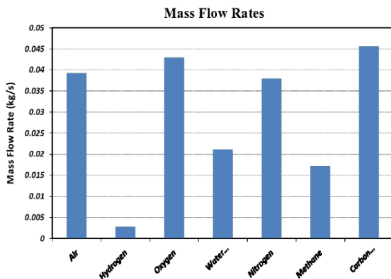
Figure 7. Comparison of Mass Flow Requirement for Various Gases.
