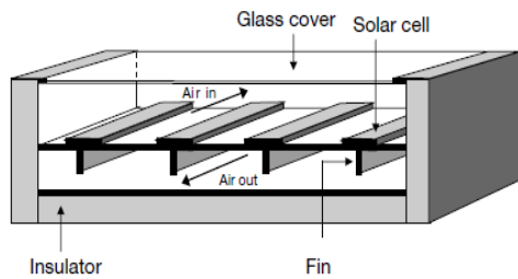
Figure 2. Finned Double-Pass Photovoltaic-Thermal Solar Air Heater [12]
