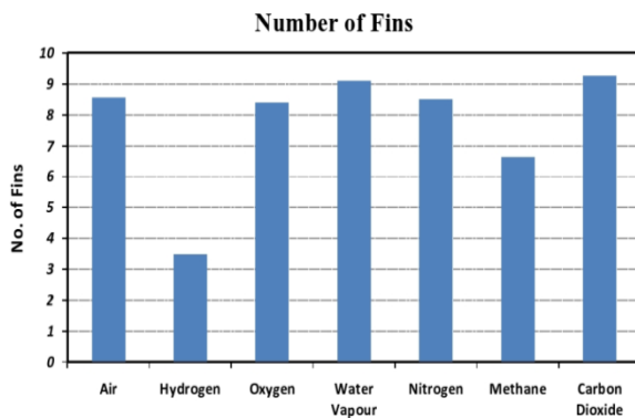
Figure 8. Comparison of Number of fins required for Various Gases.
