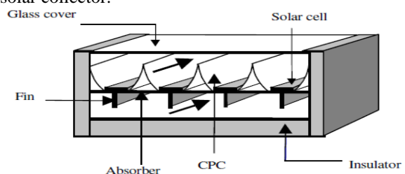
Figure 1. The Schematic Model of Single Pass, Double Duct (PV/T) Solar Collector with CPC and Fins [8]
