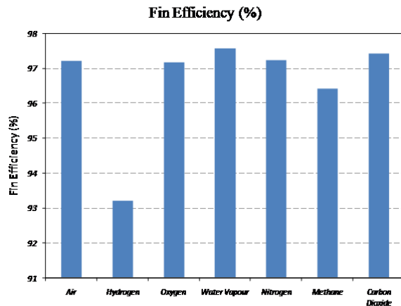
Figure 6. Comparison of Fin Efficiency for Various Gases.
