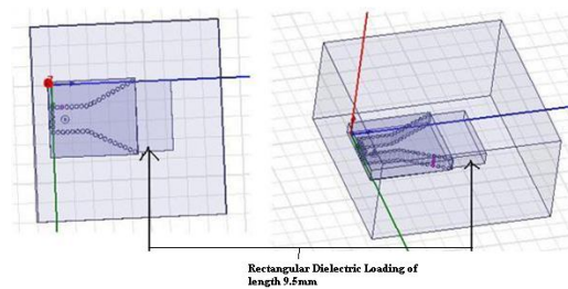
Fig 6 Short length SIW H-plane horn antenna with dielectric loading
