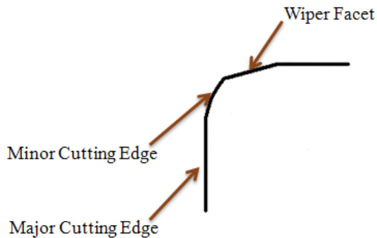
Fig. 2. Cutting edge and Wiper facet
