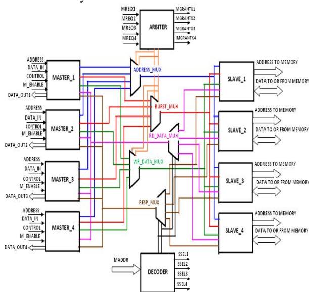
FIGURE1: Bus Architecture
