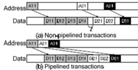
FIGURE4: Pipelined transactions
