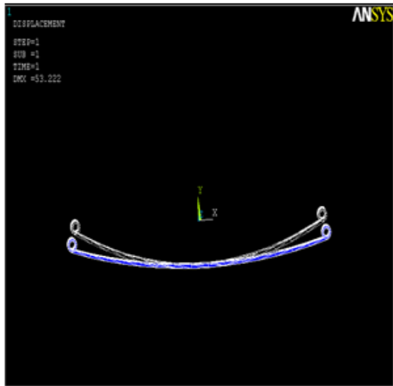
Fig.6 : Deflection of Master Leaf (Steel)
