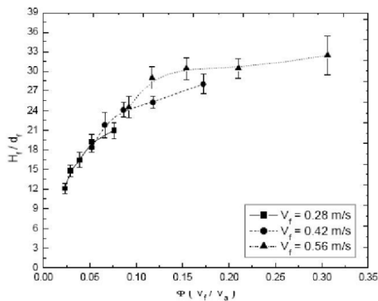
Fig.4.Variation of luminous flame length with air jet momentum for V_f = 0.28 m/s, 0.42 m/s, 0.56 m/s
