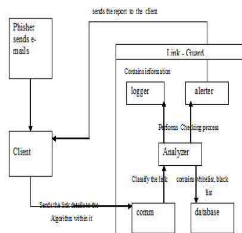
Fig 3 LINK GUARD ALGORITHM
