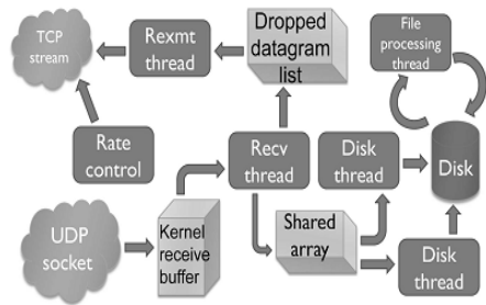
Figure 4.2 PA-UDP: the data receiver
