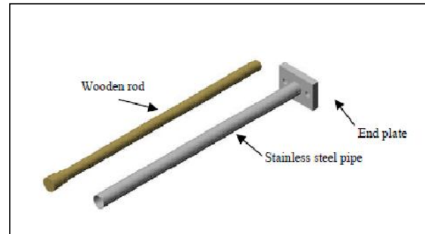
Fig. 2. Arrangement of composite cylindrical beam
