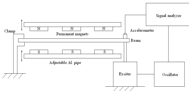
Fig. 3 (a) Block diagram of experimental setup
