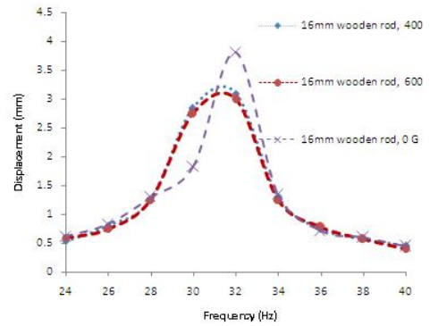
Fig. 7 Vibration spectra for composite cylindrical sandwich beam with 16 mm wooden rod
