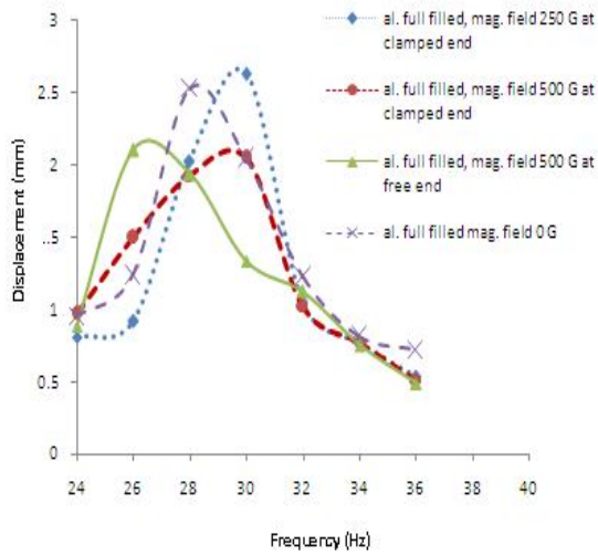
Fig. 4 : Vibration spectra for fully filled beam
