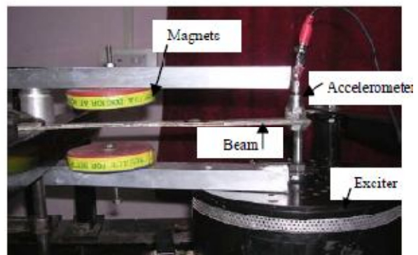
Fig. 3 (b) Photograph of experimental setup
