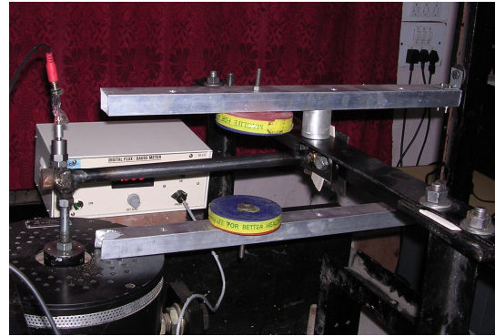
Fig. 6 Photograph of experimental setup of cylindrical composite beam
