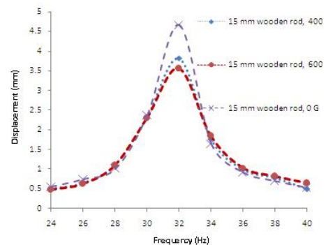
Fig. 8 Vibration spectra for composite cylindrical sandwich beam with 15 mm wooden rod
