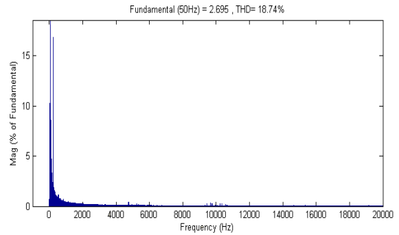
Fig (7) Simulated Results Of %THD for single inverter fed (Top trace) and dual inverter fed (Bottom trace) Induction motor drive for a modulation index of 0.4
