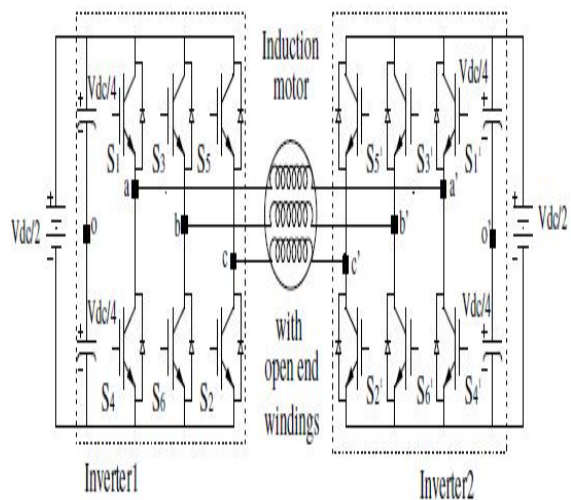
Fig (1). Power circuit configuration of dual two-level inverter
