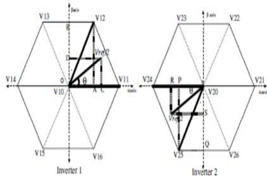
Fig. 3. Principle of decoupled PWM technique and switching voltage vector, reference voltage vector projections on \alpha and \beta axis
