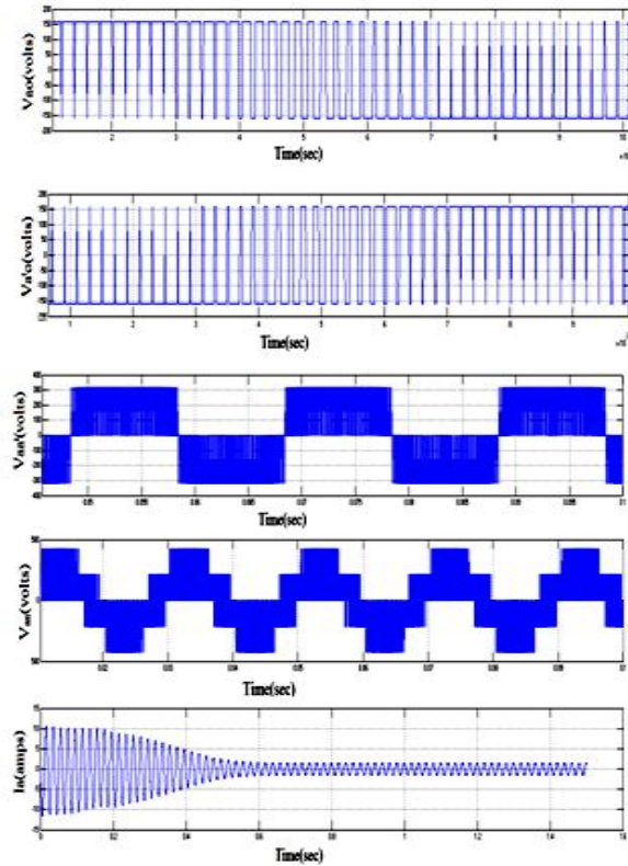
Fig (6) .Simulated pole voltages of inverter-1 and inverter-2 (Top 2 traces), Difference in a-phase pole (Vaa) voltages (3rd trace), a-phase motor phase voltage (4th trace), motor a-phase current (5th trace), for a modulation index of 0.4
