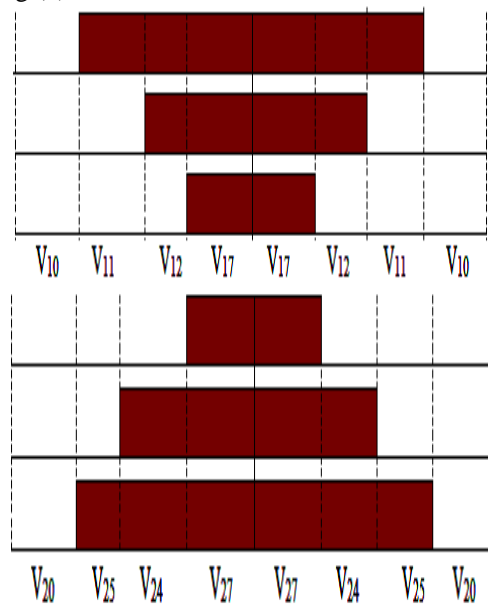
Fig (4) Switching Pattern for Inverter 1 and Inverter 2
