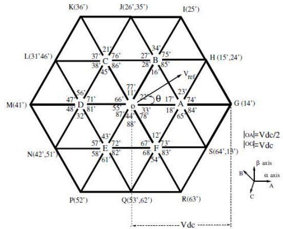
Fig. 2. Space vector locations of dual two-level inverter
