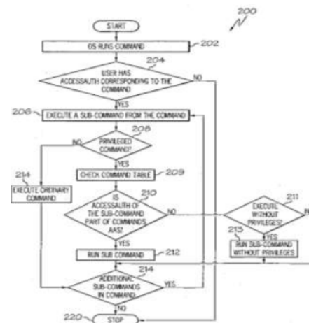
Fig 4.3 FLOW CHART FOR RBAC
