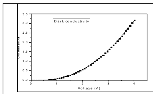
Figure 3: Dark Characteristics of Organic Solar Cell.
