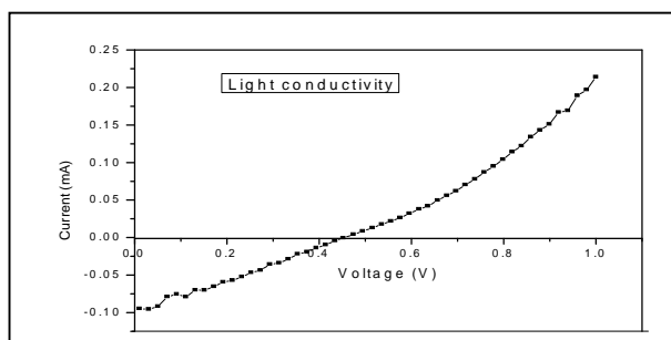
Figure 4: Light characteristics of a typical non annealed P3HT:PCBM solar cell fabricated (Sample 2).
