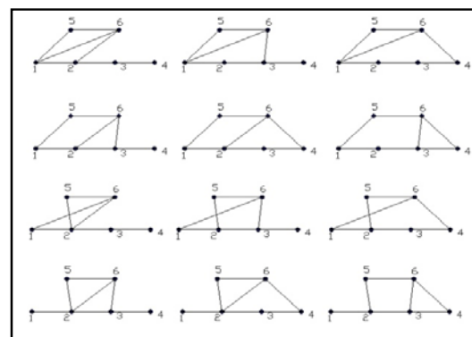
Fig. 13 : Some results of Enumeration of dependent link connection
