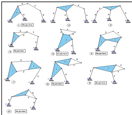
Fig. 10 : Corresponding linkage graphs for final enumeration results
