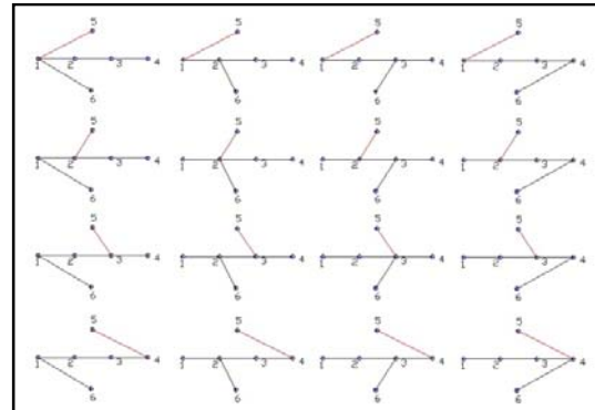
Fig.3 : Available candidates after adding the first two revolute joints for independent link connections
