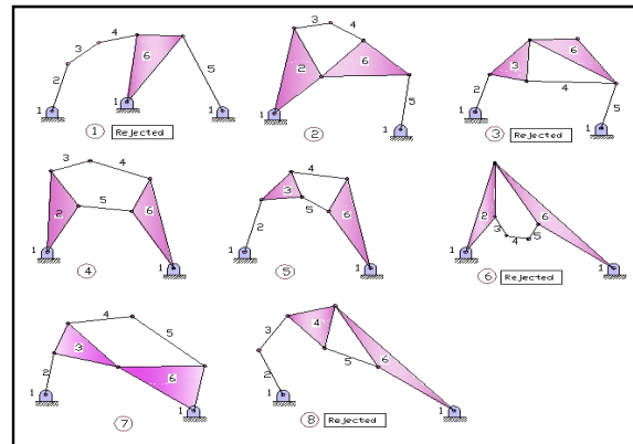
Fig. 17 : Corresponding linkage graphs for final enumeration results
