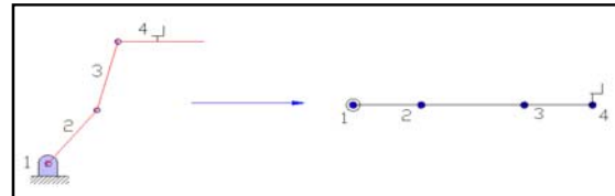
Fig. 1 : A schematic of a planar 3R robot and its corresponding graph representation
