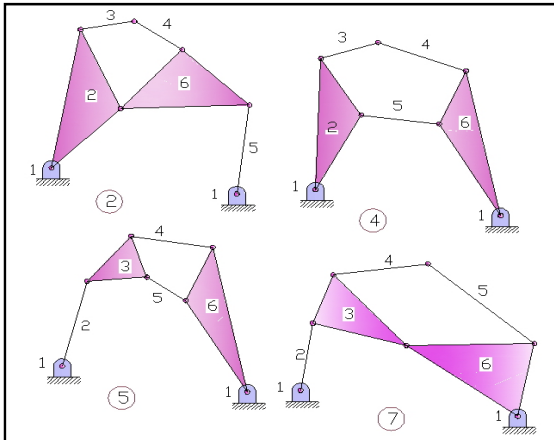
Fig. 18 : Available 6-bar mechanisms for dependent link connection
