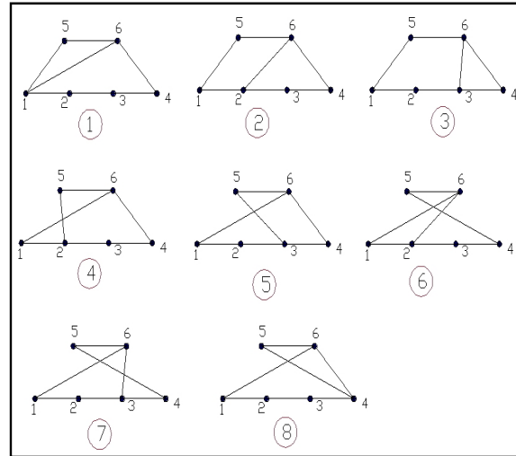
Fig. 16 : Final enumeration results for dependent link connection
