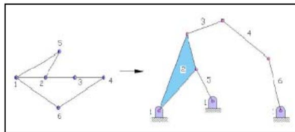
Fig. 9 : Reverse transformation process
