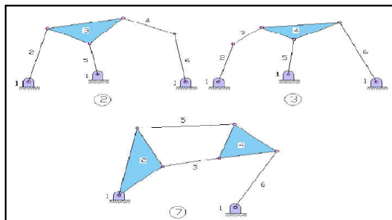
Fig. 11 : Available 6-bar mechanisms for independent link connection
