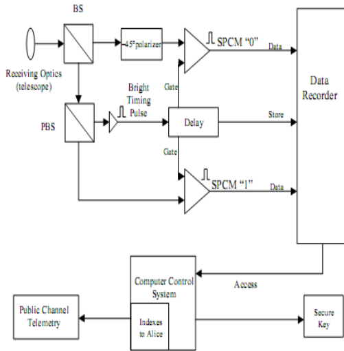
Figure 3. QKD receiver ("Bob") block diagram.
