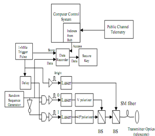
Figure 2. QKD transmitter (“Alice”) block diagram.
