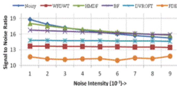
Fig. 9c SNR of Filtered Images with Gaussian Noise
