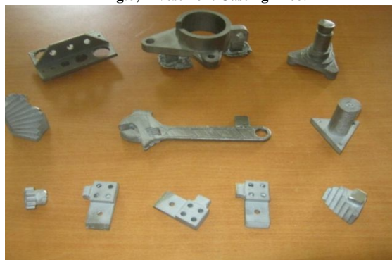
Fig.7 Castings after degating
