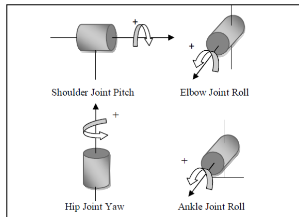
Fig. 3 : Leg and Arm Joint Structure
