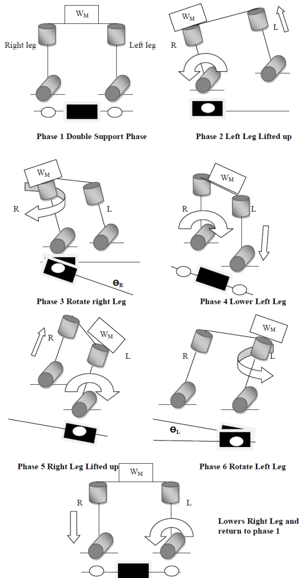
Fig. 5 : Step by step illustration of forward walking
