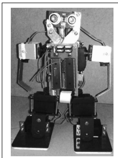
Fig. 6 : Fabricated model of the robot
