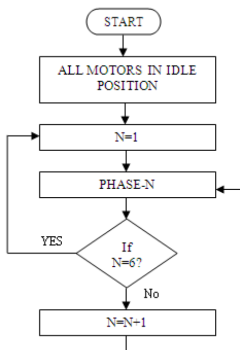
Fig. 9 : Flow Chart for forward walking
