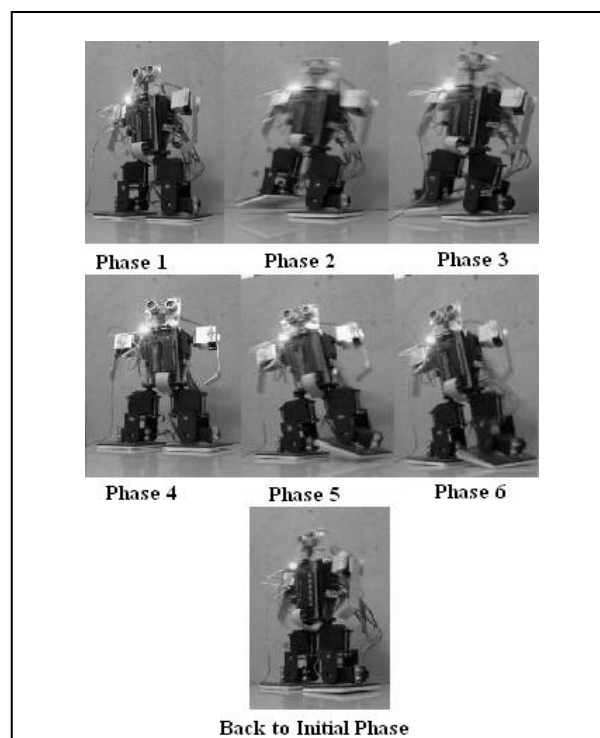
Fig. 7 : Implemented results of phases of robot gait
