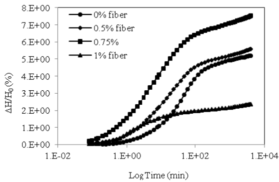
Fig. 1 : Percent swell of soil specimens versus log time with different polypropylene fibers.
