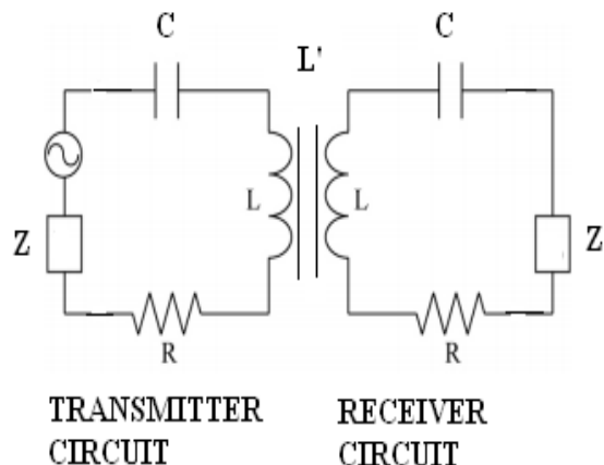
Fig. 3 Equivalent circuit of magnetic resonant coupling.
