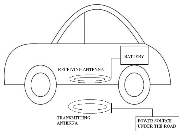
Fig. 1 Block diagram for contactless power transfer in Electric Vehicle.
