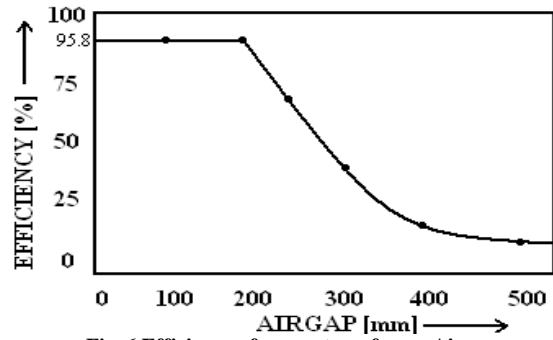
Fig. 6 Efficiency of power transfer vs. Air gap.
