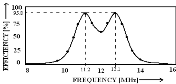
Fig. 4 Efficiency vs. Frequency at g= 100mm.
