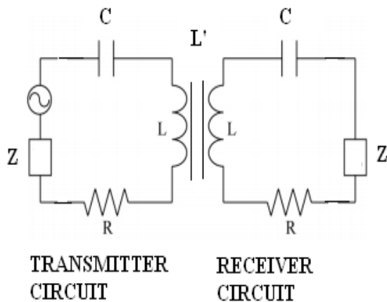
Fig. 3 Equivalent circuit of magnetic resonant coupling.
