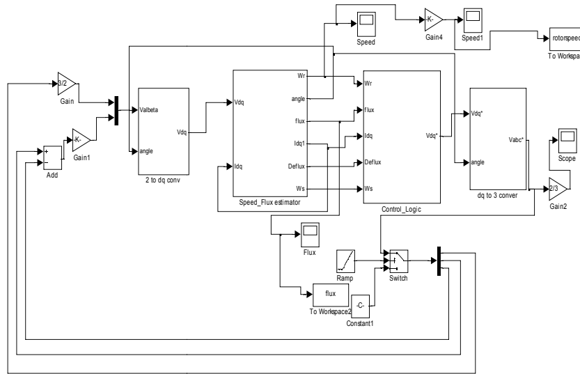
Fig1:MATLAB/Simulink model for Flux and speed estimation of Induction motor
