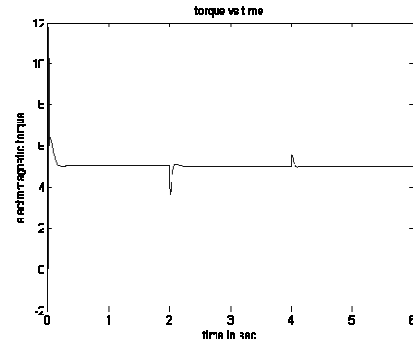
Fig5.Electromagnetic Torque
