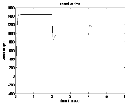
Fig2. Rotor Speed
