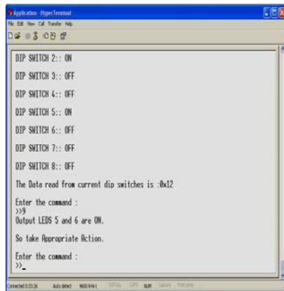
Figure 5: HyperTerminal Screen Showing Status of Certain Dip Switches and Indicating Necessary Actions Taken
