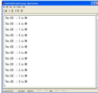
Figure 3: HyperTerminal Output Screen Showing status of Dip Switches and ADC Read Value
