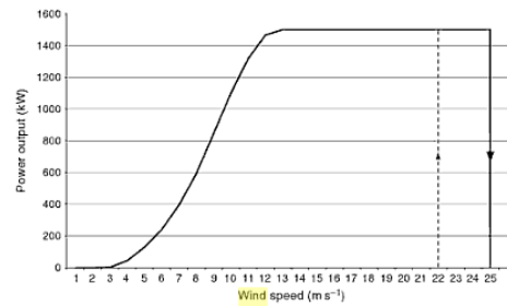
Fig1.2:- Typical power curve of a 1500 KW pitch regulated wind turbine with a cut-out speed of 25 ms -1 ( the broken line shows hysteresis effect)
