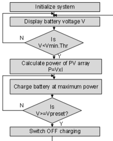
Fig. 2.3 Software design
