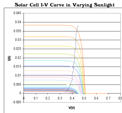
Fig. 1.1 Solar cell I-V characteristics
